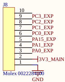
EXP1 - ADC / PWM HEADER
