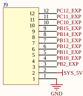
EXP2 - GPIO HEADER
